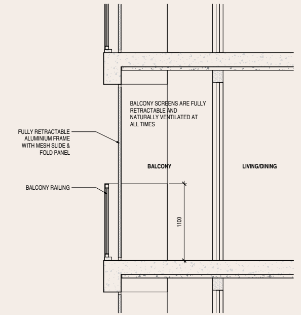
TYPICAL RETRACTABLE BALCONY SCREEN SECTION
